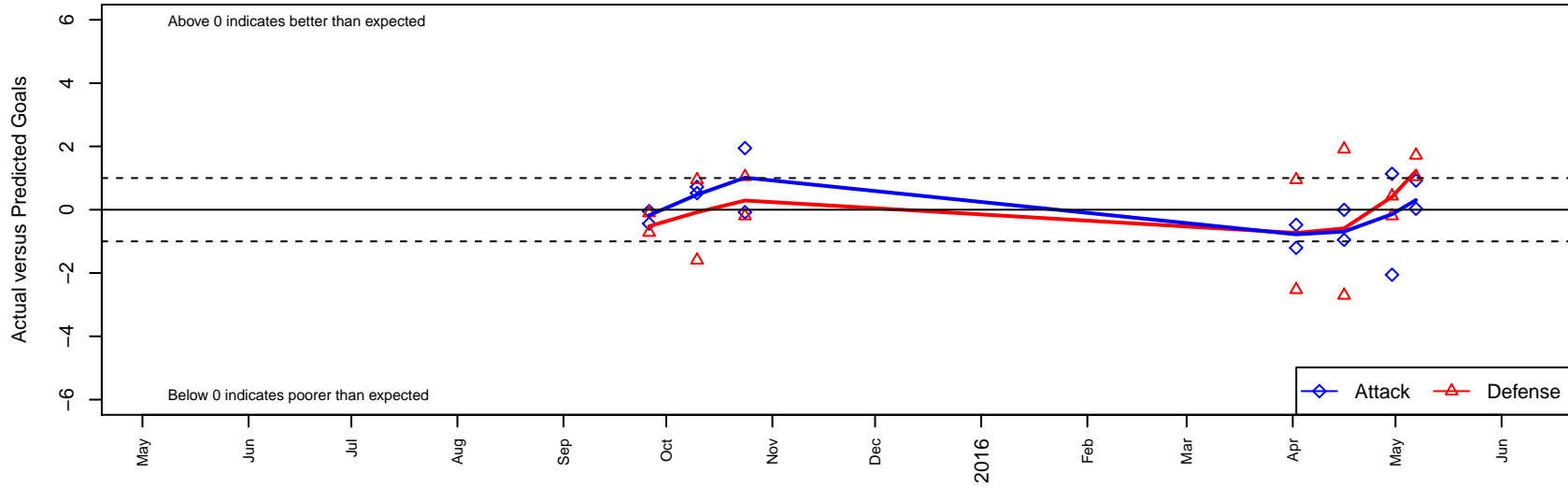
UC United B03 Dots are actual minus expected GF (blue circles) and GA (red triangles). Blue line is smoothed change in attack strength. Red is smoothed change in defense strength.
